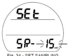
Fig. 34 - SET SAMPLING
